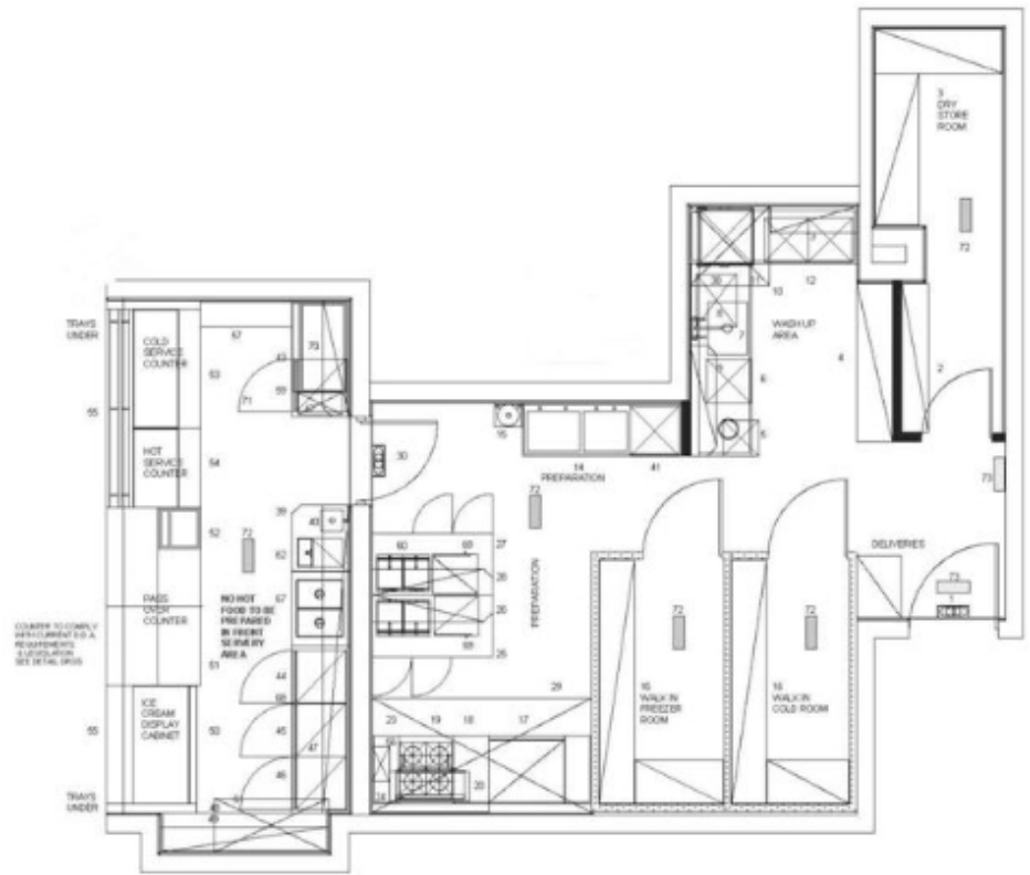
GROUND FLOOR PLAN LAYOUT
